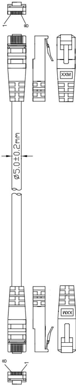
RJ45 8P8C PLUG (WHITE COLOR)
