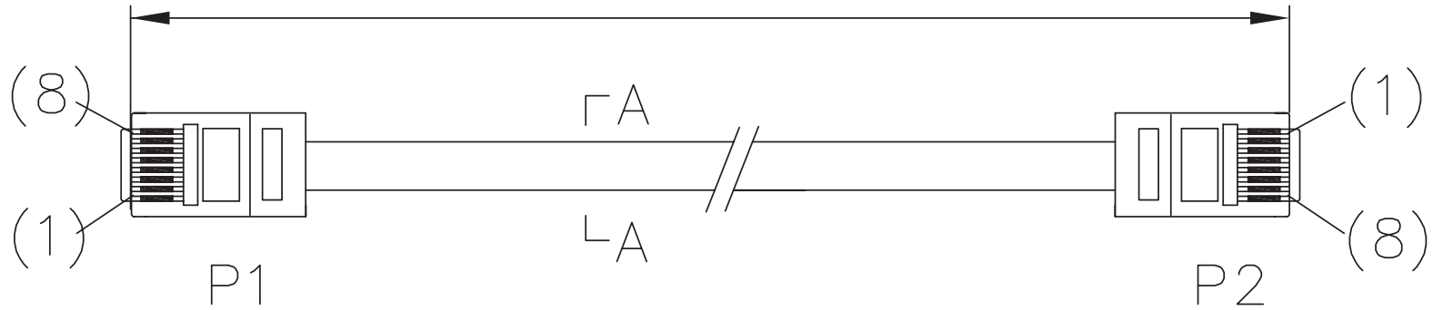
Connecting T568B
